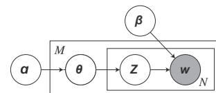
Fig. 5. Latent Dirichlet Allocation (LDA) model.
